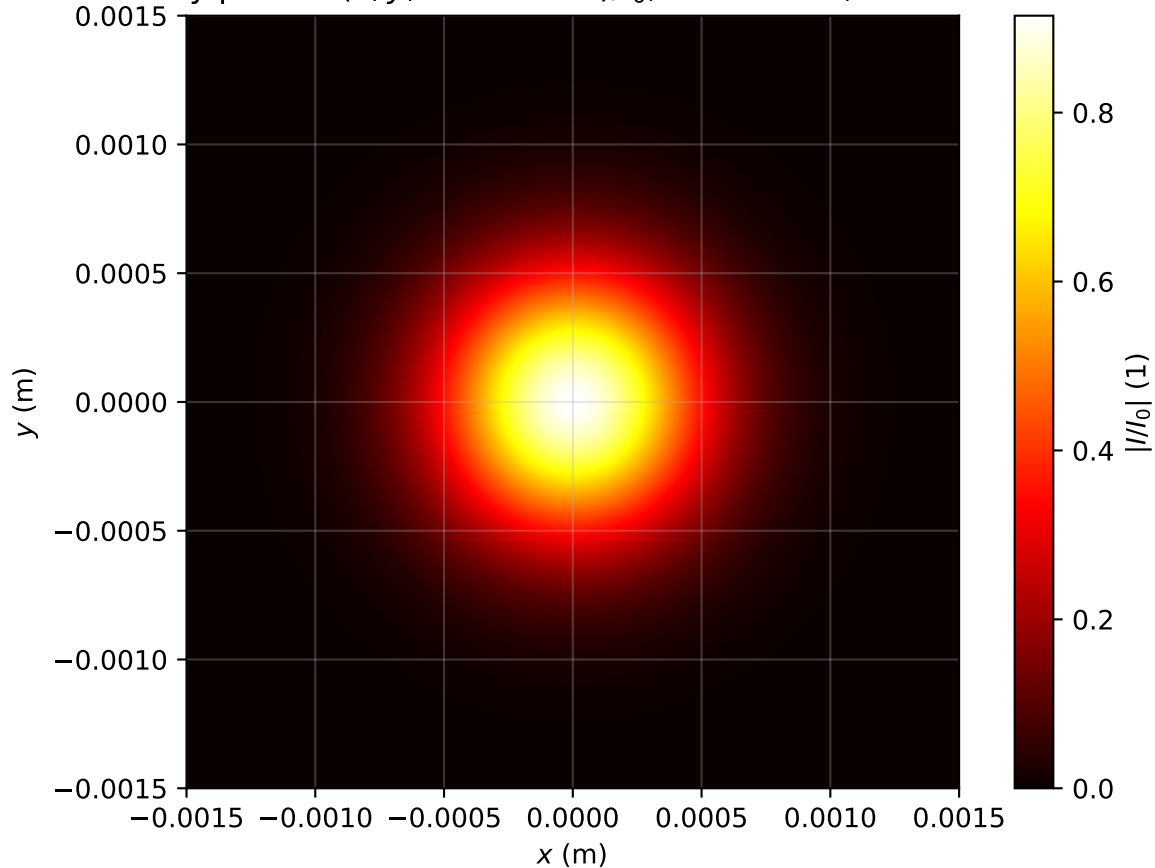
Intensity profile I(x, y, z = 0.716m)/I_0 , Pin=0.1Pcr, artificial time
